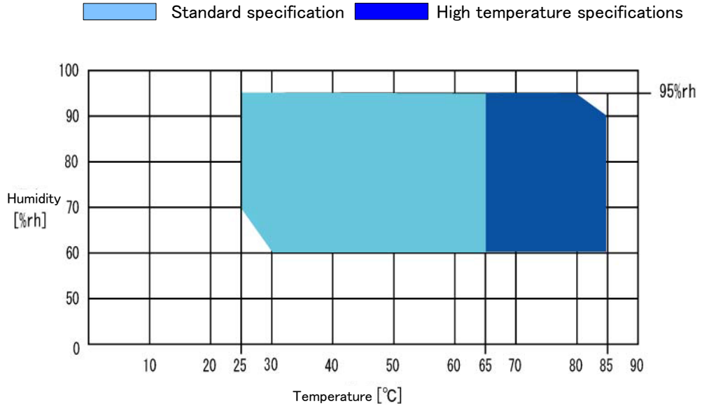
Temperature and Humidity Control Range Diagram
